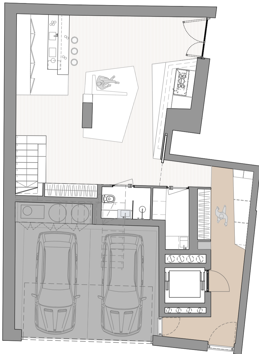
Planta entrada / Entrance floor
